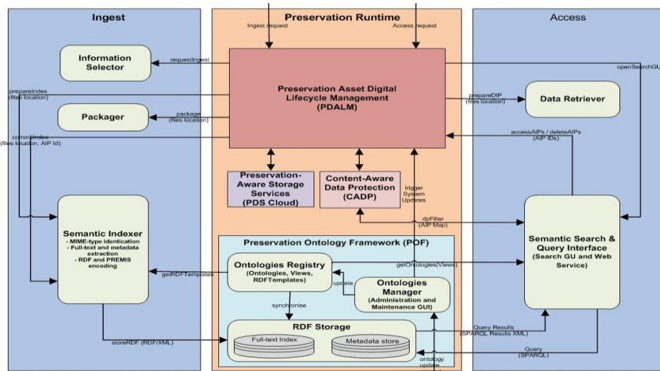
Information preparation architecture with Preservation Ontology Framework.
